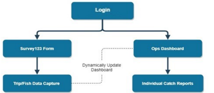
Fig. 1: Structure of the IMREC Online Diary
